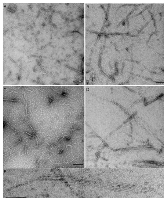
FIGURE 8: Electron microscopy images of uranyl acetate stained FtsZ filaments in the absence and presence of ZapA in 50 mM HEPES, pH 7.5, and 50 mM KCl buffer at 30 ^{\circ} C. The FtsZ concentration was 8.3 \mu M, and the reaction was initiated with 0.2 mM GTP. After 15 s a sample was removed from the reaction mixture and applied on an EM grid. FtsZ in the presence of 5 and 10 mM MgCl_2 (A and B, respectively). FtsZ filaments in the presence of 4.1 \mu M ZapA and 5 and 10 mM MgCl_2 (C and D, respectively). An enlargement of a parallel array of FtsZ filaments from a sample with 4.1 \mu M ZapA in the presence of 10 mM MgCl_2 (E). The bar equals 200 nm.
