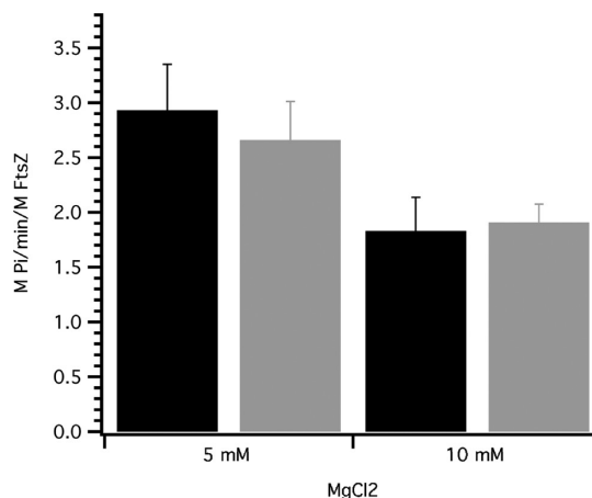
FIGURE 6: GTPase activity of 8.3 \mu\text{M} FtsZ in HEPES buffer, pH 7.5 (black), or MES buffer, pH 6.5 (gray), in the presence of 5 or 10 mM \text{MgCl}_2 as indicated. The data show the average of five experiments. The phosphate release was measured using 0.2 mM 7-methylguanosine as fluorescent marker (excitation at 300 nm) and 0.3 unit/mL purine nucleoside phosphorylase (PNP). After recording a baseline for several minutes, polymerization was induced by addition of 0.2 mM GTP. Release of phosphate from GTP hydrolysis was measured by the decrease in fluorescence at 390 nm. The determination of the initial velocity of the reaction was based on the slopes obtained by linear regression of the experimental data of the first 100–150 s. Using the same buffer conditions, a range of phosphate concentrations was used to calibrate the GTPase activity.
