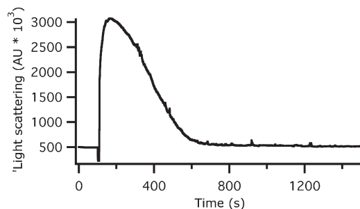
FIGURE 5: Light scattering of FtsZ polymerization (8.3 \mu\text{M} ) in MES buffer, pH 6.5, and 10 mM \text{MgCl}_2 induced with 0.03 mM GTP at 30 °C in the presence of 2 \mu\text{M} ZapA. The polymers are able to depolymerize within 1200 s in this buffer if the GTP concentration is reduced from 0.2 to 0.03 mM.
