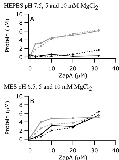
FIGURE 3: Quantification of the proteins in a pelleting assay shows that ZapA precipitates FtsZ effectively in the presence of 10 mM \text{MgCl}_2 and to a much lesser extent in the presence of 5 mM \text{MgCl}_2 . FtsZ (10 \mu\text{M} ) was incubated in prewarmed MES buffer, pH 6.5, or HEPES buffer, pH 7.5, of 30 °C with increasing ZapA concentrations. Polymerization was initiated by the addition of 1 mM GTP and allowed to continue for 2 min before the polymers were pelleted by airfuge. Supernatant and the pellet were applied on a 15% SDS–PAGE, which was stained with CBB. The stained gel was imaged, and the amount of material present in the supernatant and the pellet was determined by densitometry. The protein concentration was plotted as a function of the ZapA concentration added to the sample. Panel A: Quantification of the pellets of the CBB stained gels of the experiments in HEPES buffer, pH 7.5. Panel B: Quantification of the pellets of the experiment in MES buffer, pH 6.5. Solid lines are from the FtsZ in the pellet and dashed lines from the ZapA in the pellet. Black and gray lines are from the experiments in the presence of 5 and 10 mM \text{MgCl}_2 , respectively. The corresponding CBB stained gels are shown in Supporting Information Figure S1.
