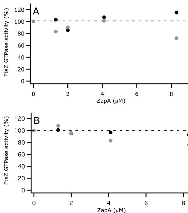
FIGURE 7: ZapA seems not to affect the GTPase activity of FtsZ dramatically. FtsZ (8.3 \mu M) was preincubated with various ZapA concentrations at 30 ^{\circ} C in HEPES buffer, pH 7.5 (A), or in MES buffer, pH 6.5 (B), in the presence of 5 mM MgCl_2 (black markers) or 10 mM MgCl_2 (gray markers), with 0.2 mM 7-methylguanosine (excitation at 300 nm) and 0.3 unit/mL PNP. After recording a baseline for several minutes, polymerization was induced by addition of 0.2 mM GTP. Release of phosphate from GTP hydrolysis was measured by the decrease in fluorescence at 390 nm. The initial velocity of the reaction was fitted by linear regression as described in the legend of Figure 6, and the slope was plotted on the Y-axis as percentage of the activity of FtsZ in the absence of ZapA obtained from Figure 6.
